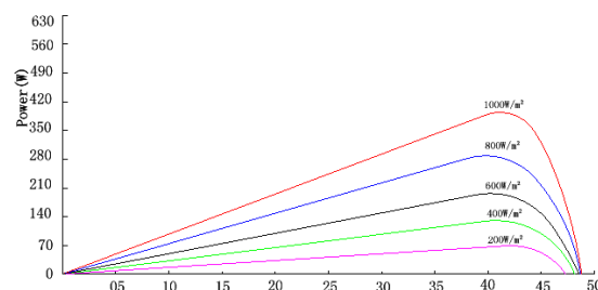
P-V Curves of PV Module GEO-PM10-54S400w
