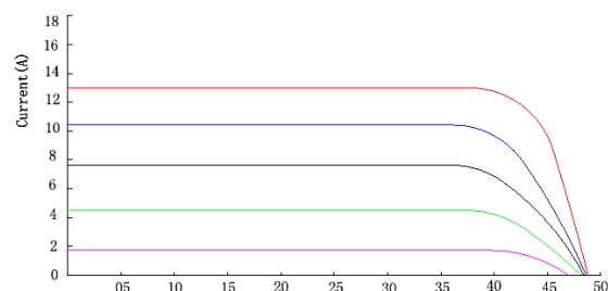
I-V Curves of PV Module GEO-PM10-54S400w
