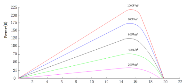
P-V Curves of PV Module BM10-28S225W
