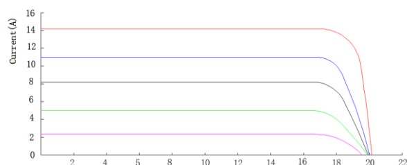
I-V Curves of PV Module BM10-28S225W
